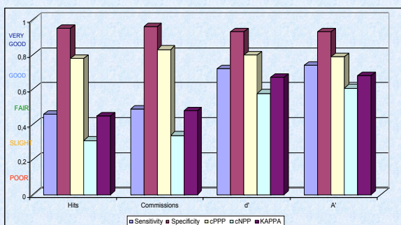
FIGURE 2. Statistical Indexes of CSAT Measures
